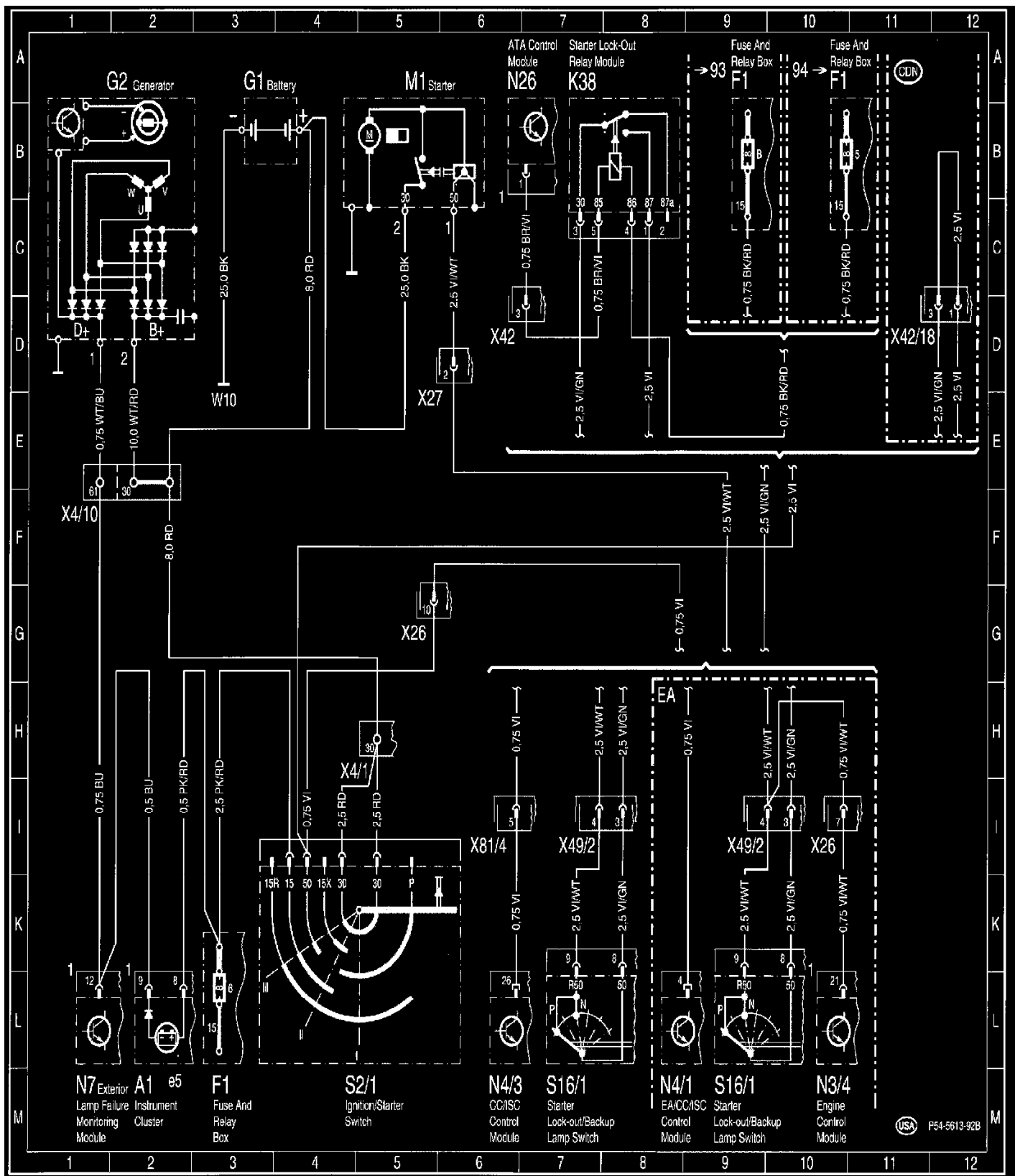
Starter, Generator, Battery
